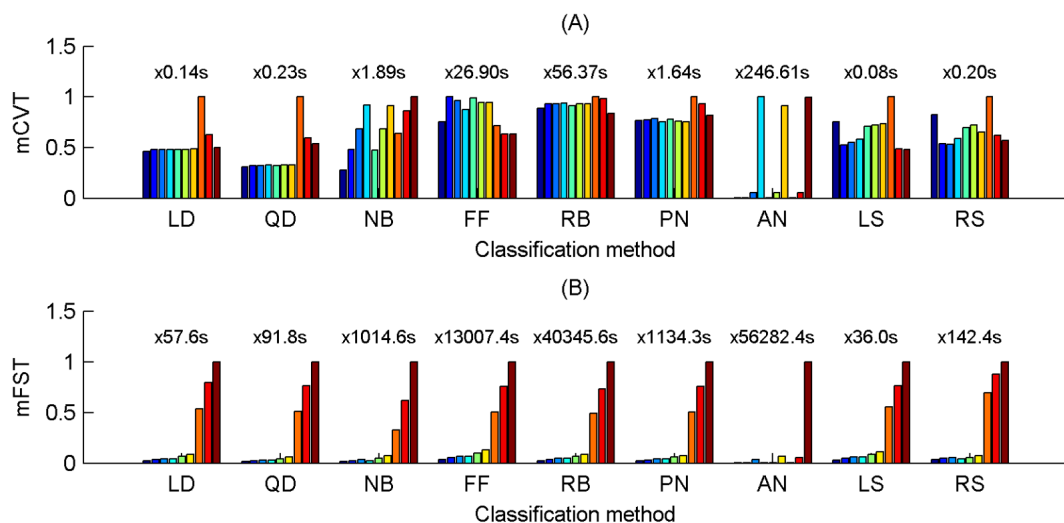
Figure 4.3. Individual-level overall median cross-validation (mCVT) and feature selection (mFST) times for all classification methods. Bars represent normalized values, real computation times in seconds can be obtained using multiplication factors presented above the bar diagrams. (A) First bars stand for cross-validations with a single input feature, 2 nd -4 th bars denote classifications with 2-4 measures of single channels, 5 th -7 th bars present results for classifications with 2-4 channels of single measures, 8 th -10 th bars stand for classifications using 2-4 measure x channel combinations as features. (B) Meaning of the bars is equal to those of 2 nd -10 th bars in (A) part of the Figure. To resolve the abbreviation of the classification methods see section 4.2.2.1.
